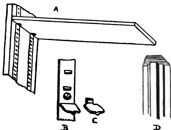
FIG. 39.—Tonks' Shelf Fittings (Section 179).
